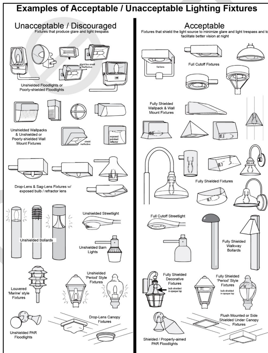
Figure IV-10: Cutoff Light Fixtures
