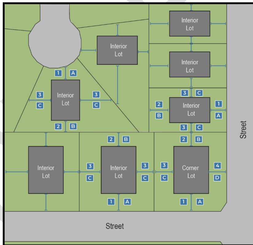
Figure IV-1: Lots, Yards, and Setbacks Summary
