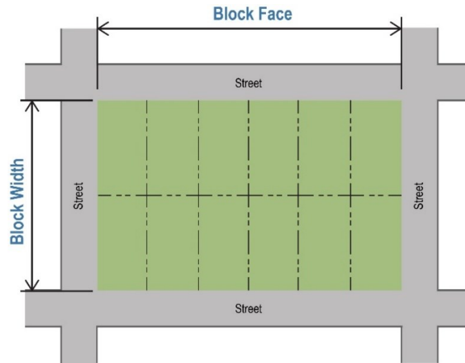
Figure V-2: Block Measurements
