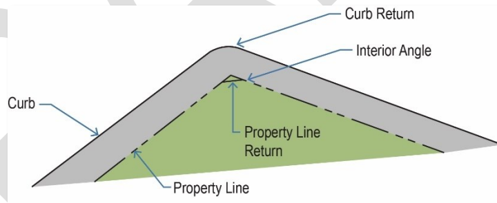
Figure V-4: L-shaped (elbow type) Intersection
