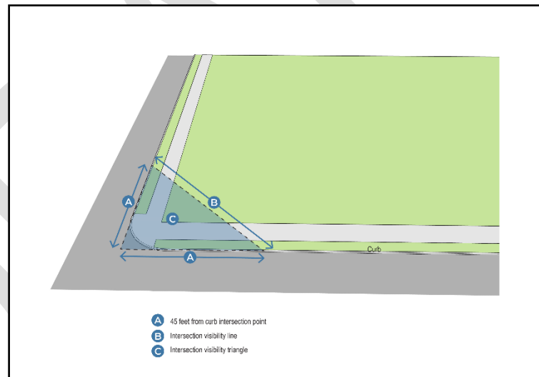
Figure IV-3: Visibility at 45' Intersection Point
