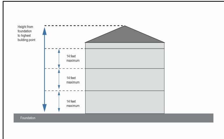
Figure IV-6: Building Height
