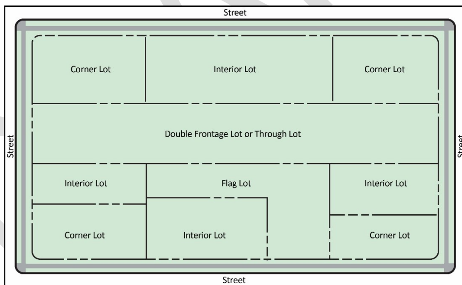
Figure V-1: Lot Types and Arrangements
