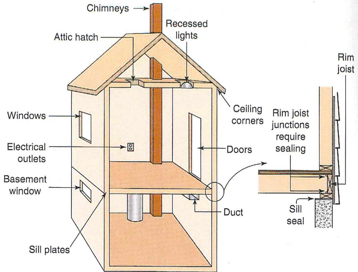
Typical sources of air leakage
