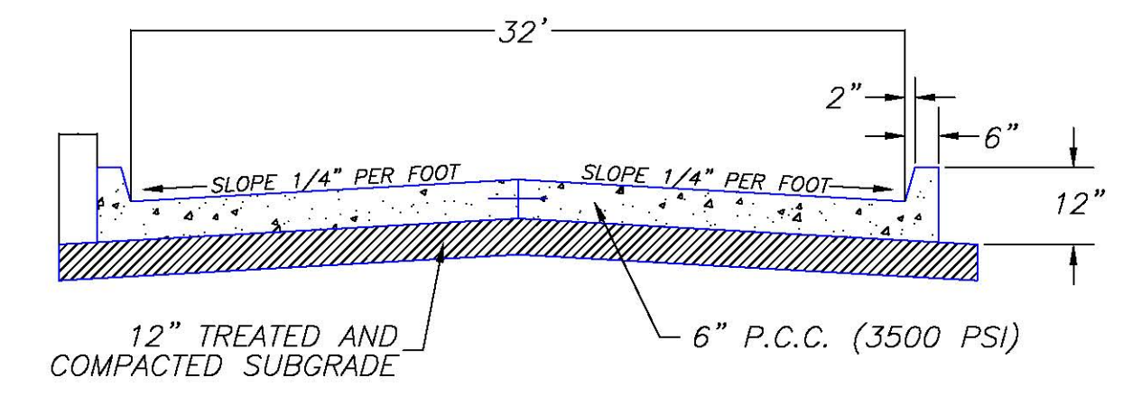
CURB & GUTTER - CONCRETE TYPICAL GRADING AND SURFACING SECTION N.T.S.
